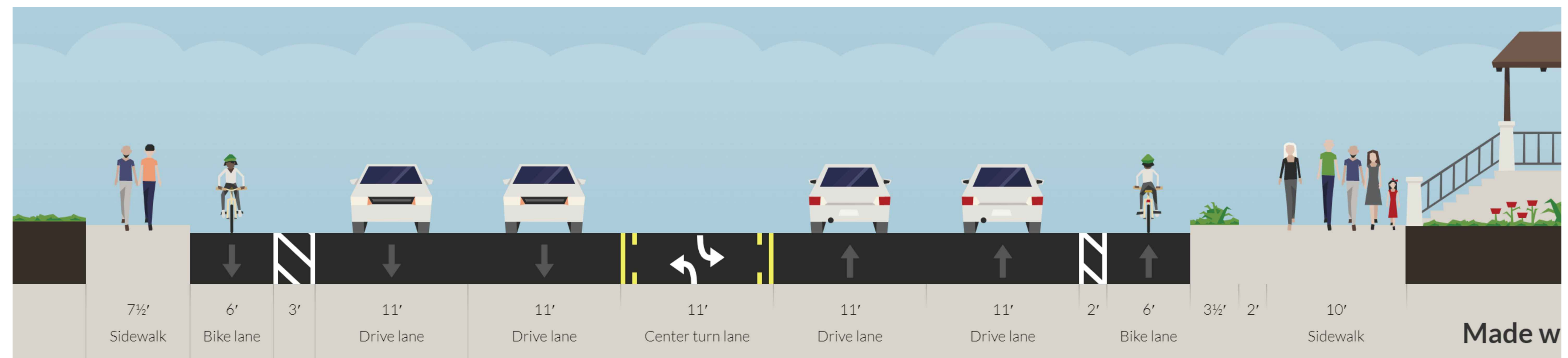
SECTION D-D: PROPOSED
