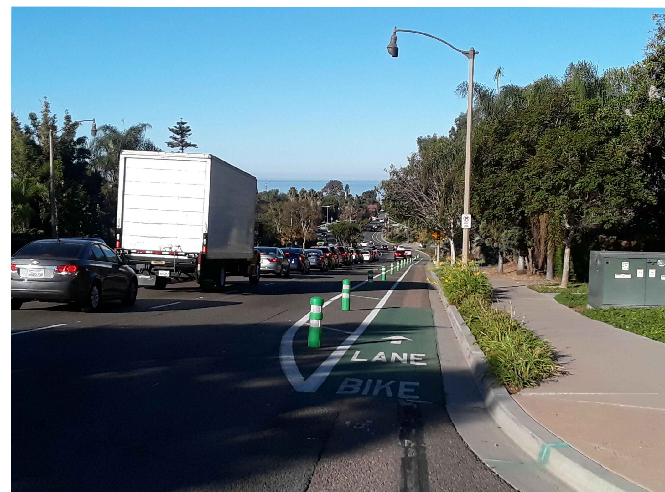
BIKE LANE CHANNELIZER EXAMPLE. PHOTO AT LEUCADIA BLVD IN ENCINITAS
