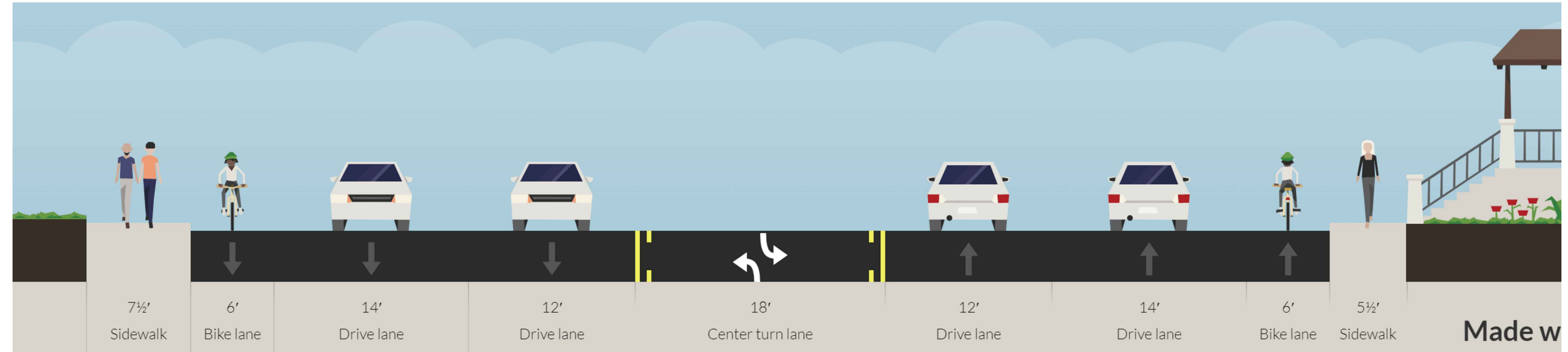
SECTION D-D: EXISTING
